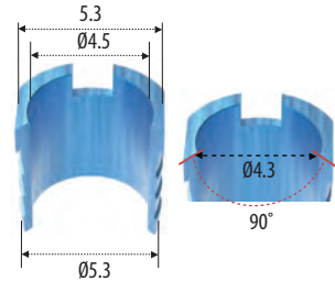
Open Sleeve KLS02
